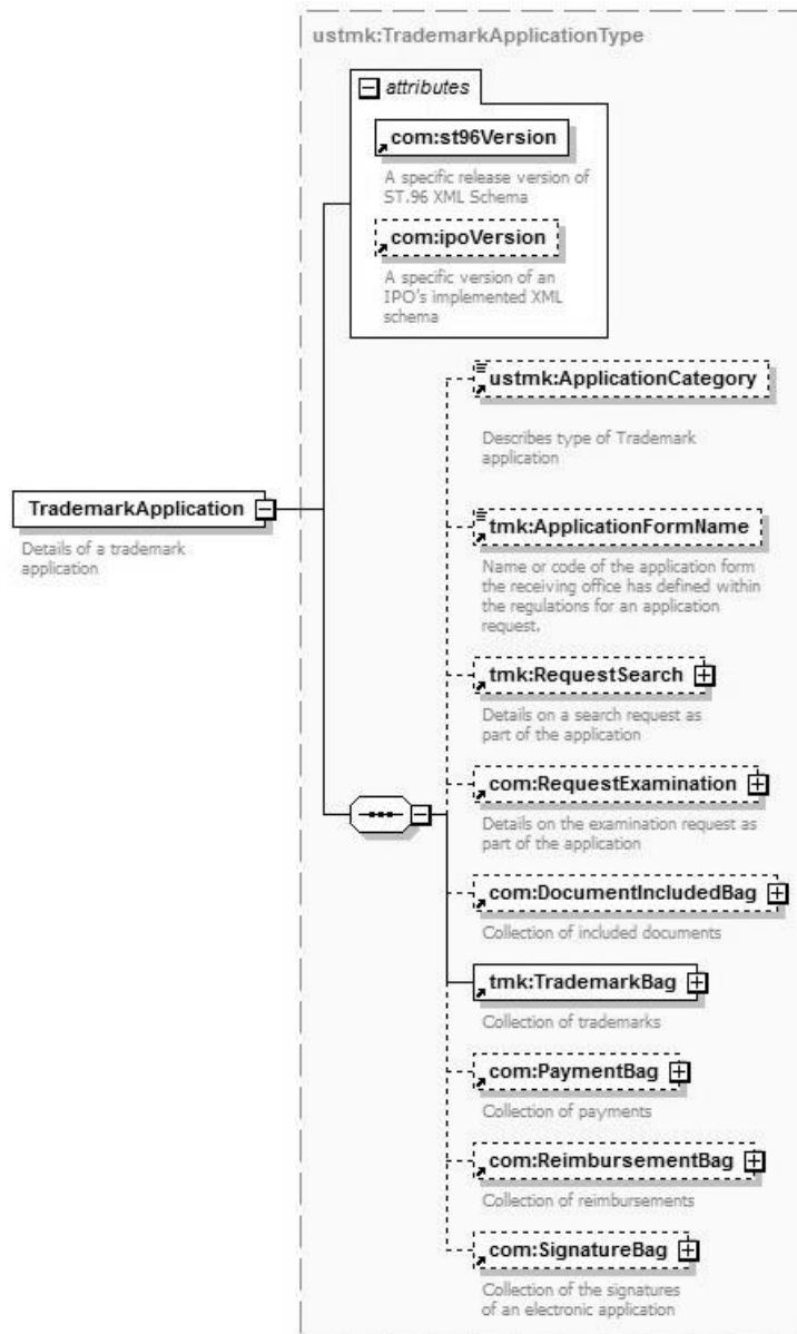
Figure 23: ustmk: TrademarkApplication
